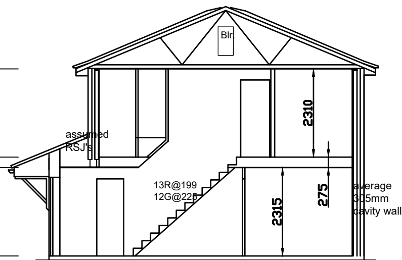
Section X-X
