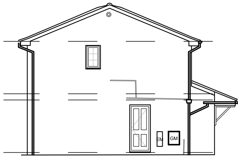
North Elevation
