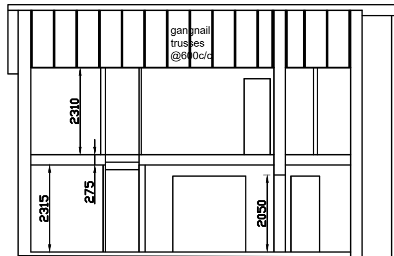
Section Y-Y
